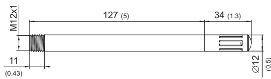
Fig. 1 Dimensions of HTP201 in mm (inch)
