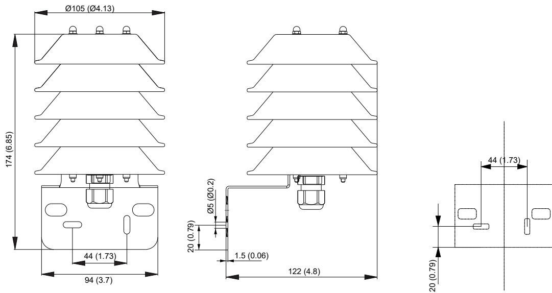
Fig. 2 Dimensions of optional radiation shield (ordering code HA010502) in mm (inch)
