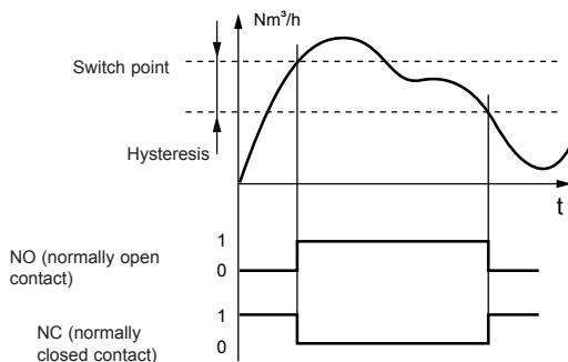
Fig. 2 Hysteresis mode
