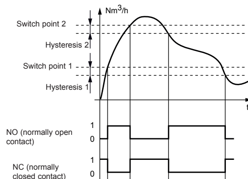
Fig. 3 Window mode
